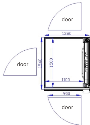
Platform dimensions and available configurations of doors.
