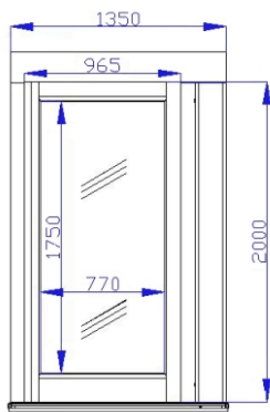
Standard panoramic single hinged door.
